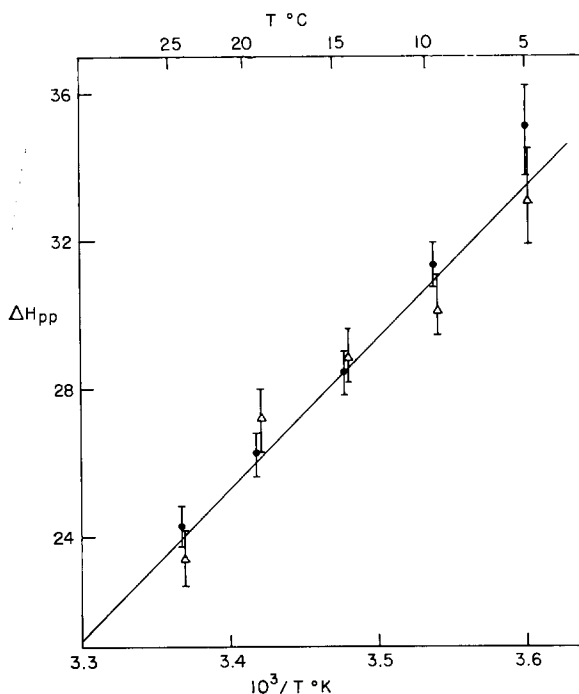
Fig. 4. Linewidth ( \Delta H_{pp} ) temperature dependence of the g = 1.98 EPR line of 3.6 \cdot 10^{-5} M MnSO_4 in 0.8 M Tris, pH 8.0 (● - - ●), and of Tris-washed chloroplasts ( \Delta - - \Delta ). To minimize denaturation effects, lower temperatures were recorded first. Instrumental conditions: Microwave power 100 mW, modulation amplitude 6.3 G. Chlorophyll content 2.80 mg/ml.
