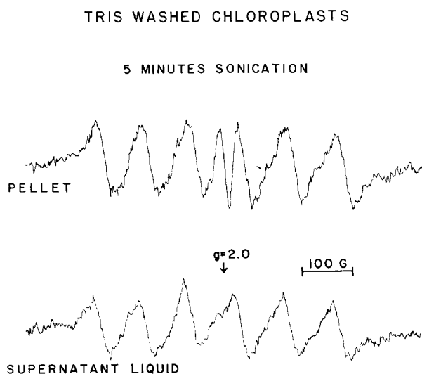
Fig. 3. Room temperature EPR spectra of sonicated Tris-washed chloroplasts. Samples were prepared as described in Materials and Methods. Instrumental conditions: microwave power 80 mW, modulation amplitude 10 G, time constant 1.0 s, scan rate 250 G/min.
